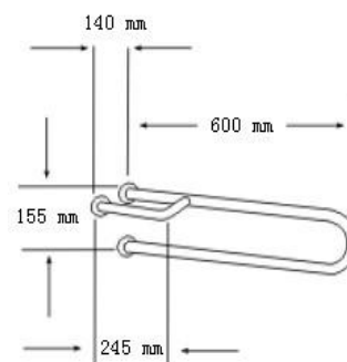
15.253.S 600 mm 15.254.S 800 mm
